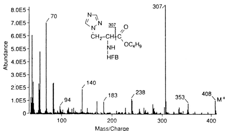
Fig. 3. Mass spectrum of triazolylalanine (heptafluorobutyryl amide, i -butylester) isolated from mature apples after application of 400 mg [3,5- 14 C]amitrole (61.3 MBq × mmol -1 ) to apple trees.
